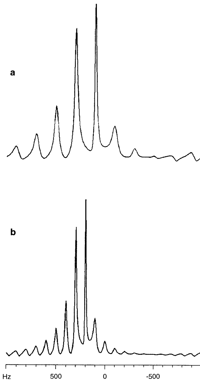
FIG. 5. Simulated spectra corresponding to those in Fig. 4 using T_{rd} = 0.012 s.
